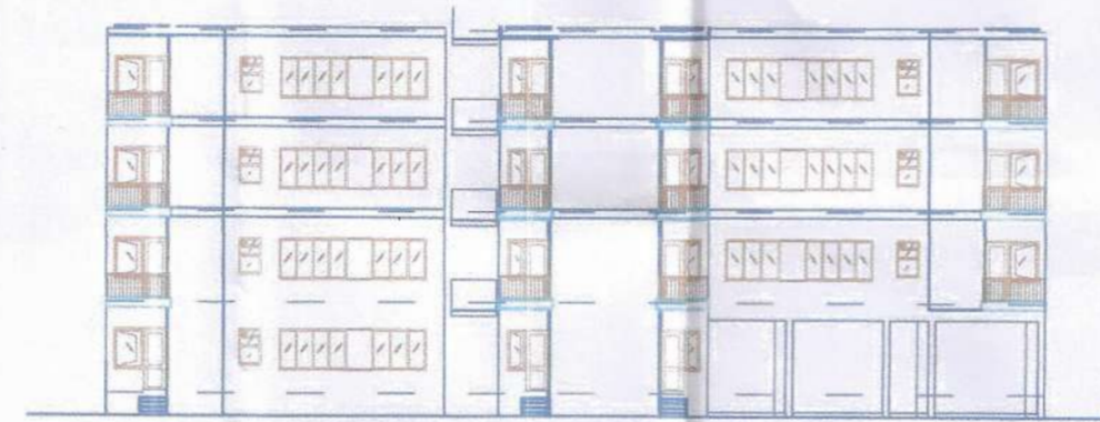
SCALE 1:200 FRONT SIDE ELEVATION
